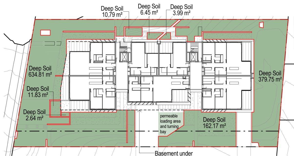
4 Deep Soil Scale 1 : 500
